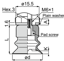
VP20, 25, 30B 5 -M6
