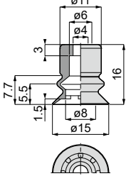
VP15B [5] Weight : 1.2g[1.9g]
