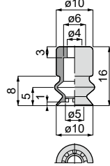
VP10B [5] Weight : 0.8g[1.3g]
