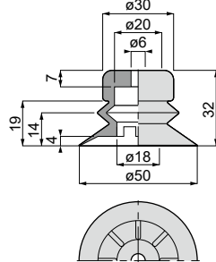
VP50B [5] Weight : 15g[22g]
