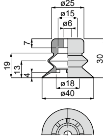
VP40B [5] Weight : 11g[17g]
