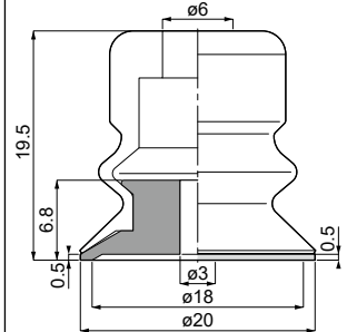
VP20B [5]- Q [8] Weight : 3.4g[4.6g]
