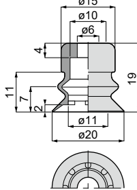
VP20B [5] Weight : 2.1g[3.3g]
