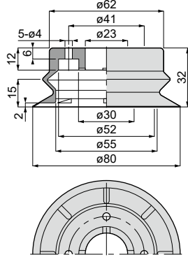
VP80B [5]-M10 (Pad & screw set)
