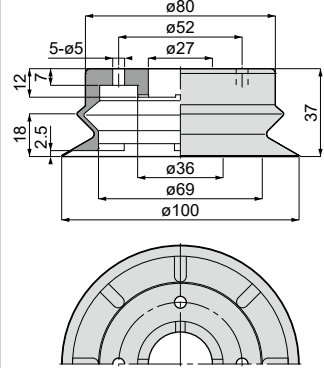
VP100B [5]-M10 (Pad & screw set)
