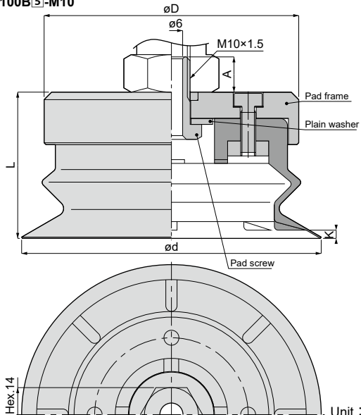
VP80, 100B 5 -M10
