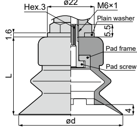
VP40, 50B 5 -M6
