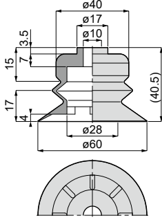
VP60B [5] Weight : 27g[43g]
