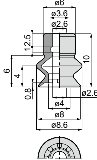
VP20B [5] Weight : 2.1g[3.3g]
