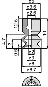
VP15B [5] Weight : 1.2g[1.9g]
