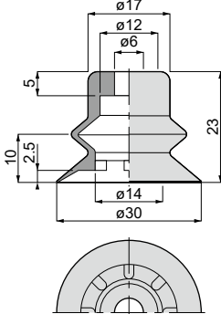
VP30B [5] Weight : 3.9g[6.2g]
