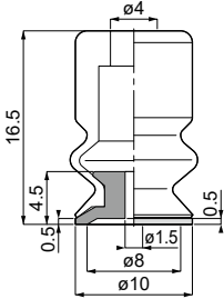
VP10B [5]- Q [8] Weight : 1.1g[1.6g]
